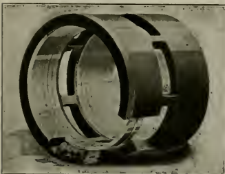
FIG. 2. VALVE CHAMBER.
